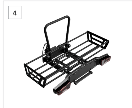
4 Transportkorb SEGSYA7200
